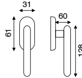
art. FI 2.1260 dk movimento in fibra
