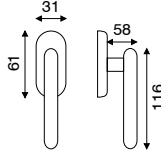
art. 4.8660 dk movimento in fibra
