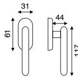
art. 4.7860 dk movimento in fibra
