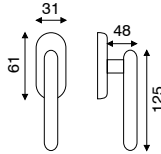
art. FI 2.1660 BIC dk movimento in fibra
