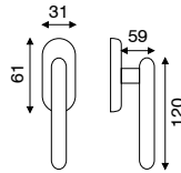
art. 4.696O dk movimento in fibra
