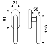
art. FI 2.286O dk movimento in fibra
