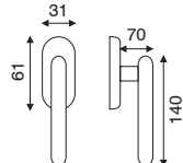
art. FI 2.5560 dk movimento in fibra
