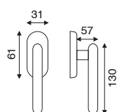
art. FI 2.1560 dk movimento in fibra
